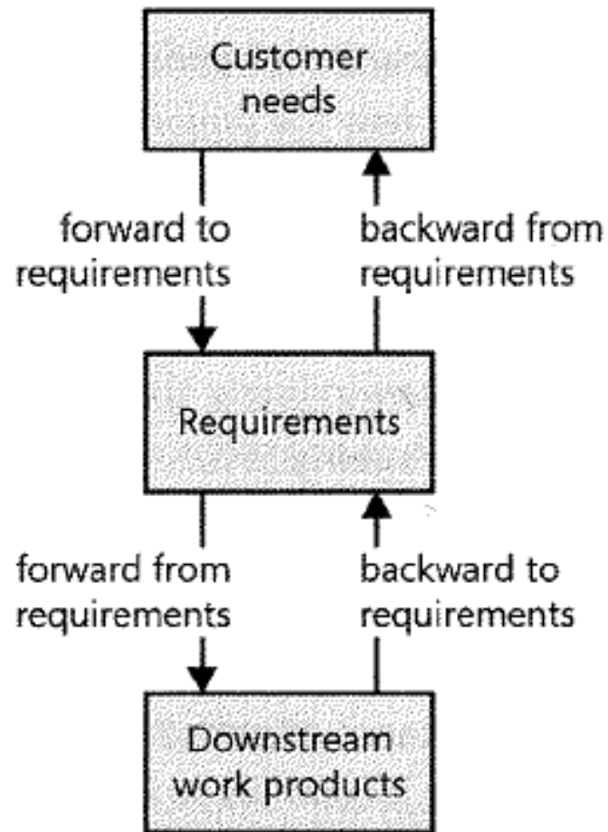
FIGURE 29-1 Four types of requirements tracing.
