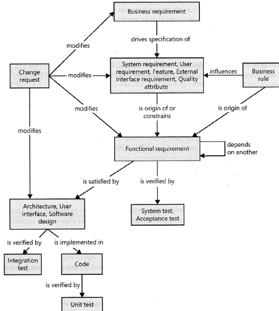
FIGURE 29-2 Some possible requirements trace links.
