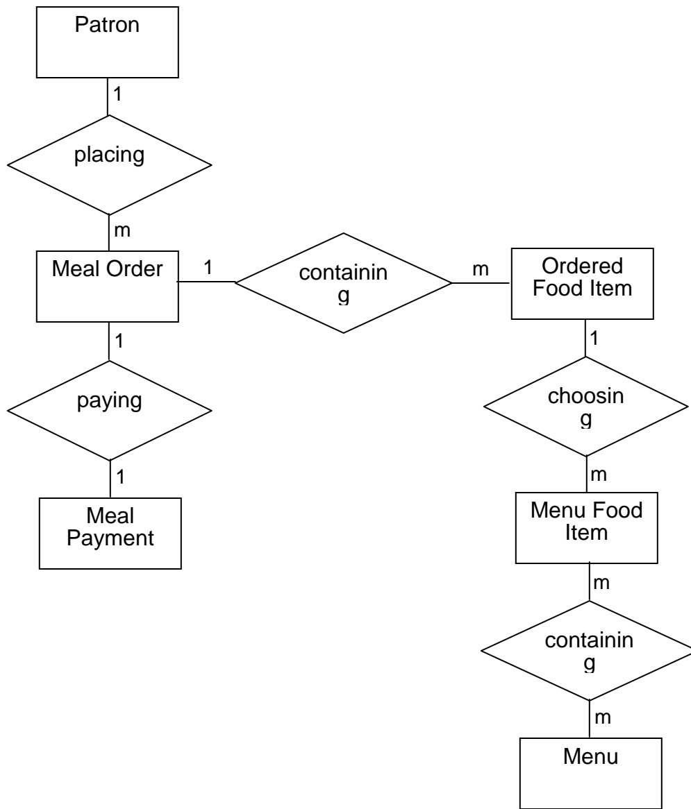
Figure 2 Partial data model for release 1.0 of the Cafeteria Ordering System.
