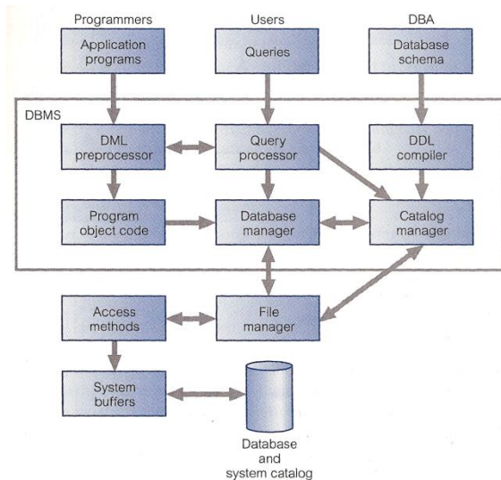
Figure 3.15 Components of a database manager.
